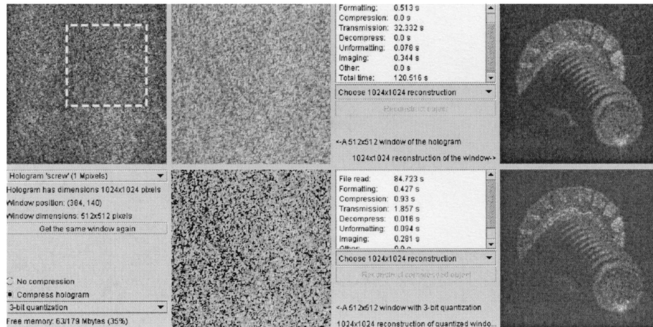
Fig. 4. Screenshot of client side of timings application. Top row (l to r): full Fresnel field with window indicated, uncompressed Fresnel field window data, uncompressed timings, and uncompressed reconstruction. Bottom row (l to r): control panel, compressed window, compressed timing information, and compressed reconstruction.
