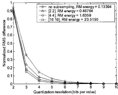
Fig. 5. NRMS difference in the reconstructed intensity plotted versus the number of bits in each of the Fresnel field's real and imaginary values for various degrees of subsampling.
