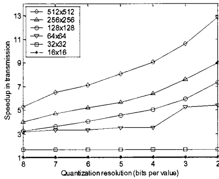
Fig. 7. Speedup as a function of increasing compression, for various Fresnel field window sizes.
