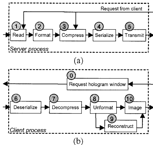
Fig. 3. Internal operation of (a) server and (b) client processes.
