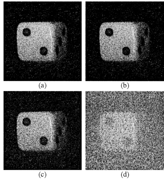
Fig. 6. Reconstructed views (with 4 \times 4 subsampling) from a 1024 \times 1024 -pixel window from the Fresnel field stored with different quantization resolutions: (a) no quantization, (b) 4 bits, (c) 3 bits, (d) 2 bits of resolution in each real and imaginary value.
