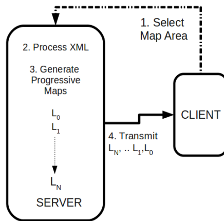
Figure 1: Schematic diagram of the implementation of our progressive transmission model
