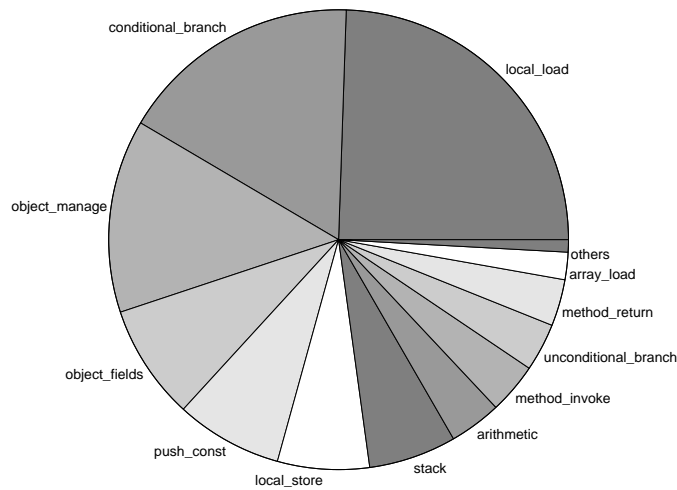
Figure 3. Total (API and Non-API) dynamic bytecode execution frequencies by category by the Eiffel programs studied when compiled using SmallEiffel no_check mode.
