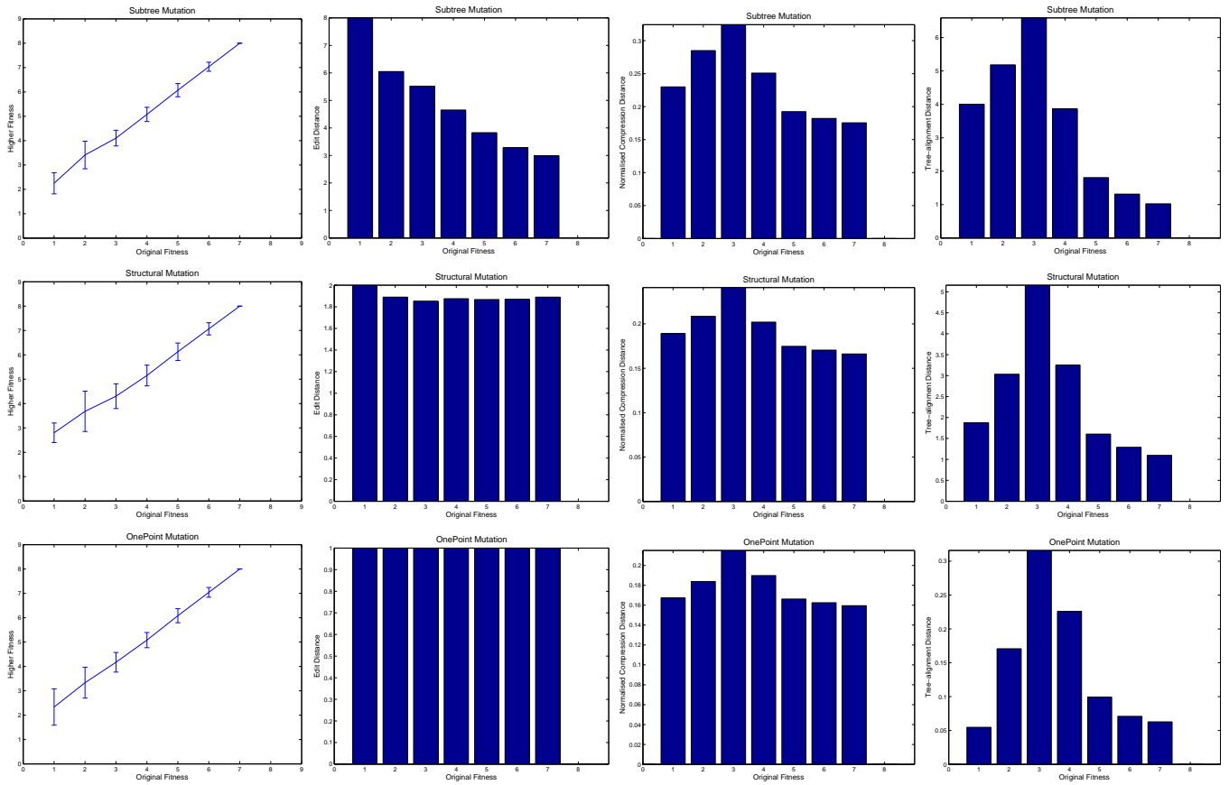
Figure 3: Results after applying subtree (top), structural (middle) and one-point mutation (bottom) using the even-3-parity problem. Original fitness versus higher fitness (first column) and distance metrics using edit (second column), normalised compression (third column) and tree-alignment distance (fourth column).
