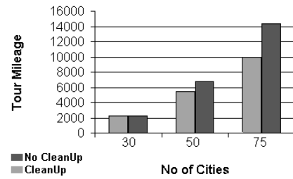
Figure 3: Effect of "Cleanup" operator
