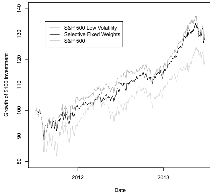
Fig. 2. Performance of various portfolios for test period
