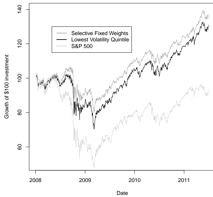
Fig. 1. Performance of various portfolios for training period
